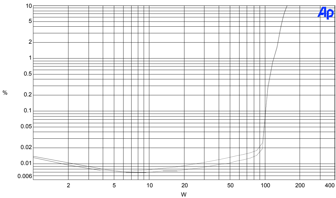
Bel Canto eVo2 THD+N vs PWR out 8 ohm load
