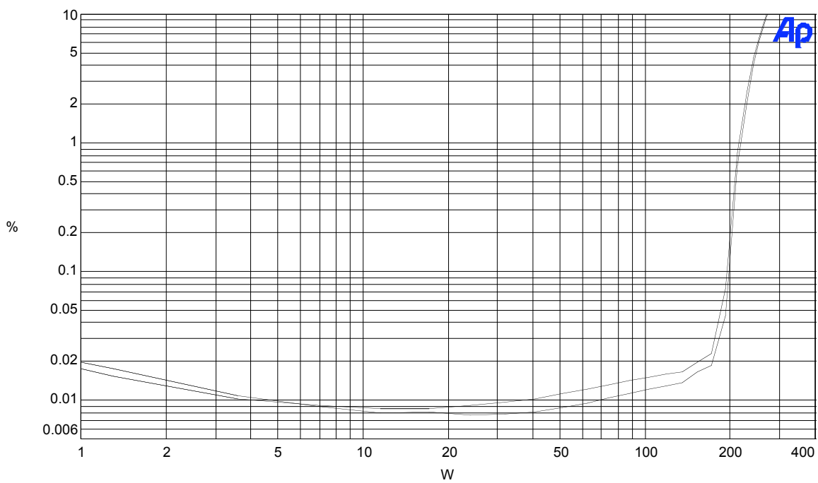
Bel Canto eVo2 THD+N vs PWR out 4 ohm load
